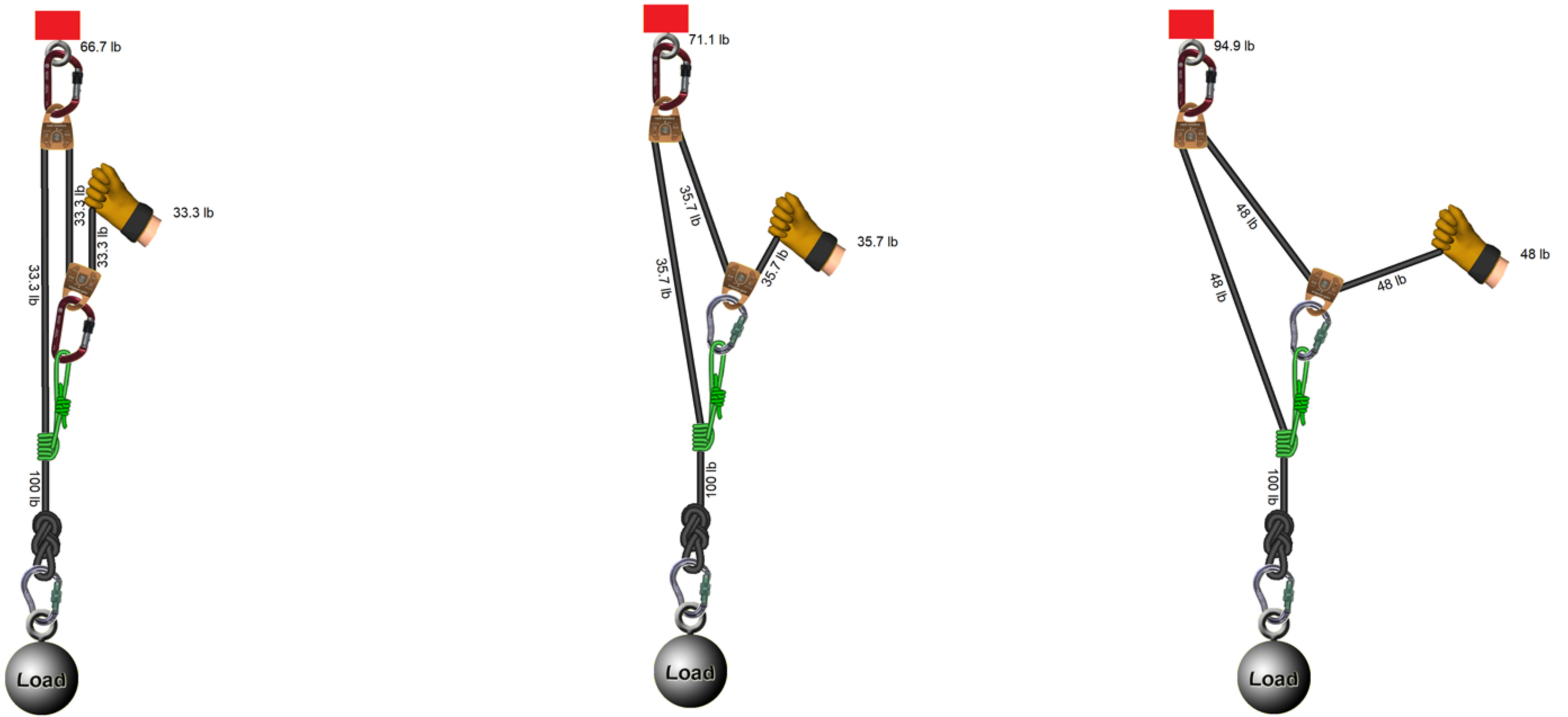
Effects of pull angle on hauling efficiency with 100 Lb. load. (System friction not being considered)
